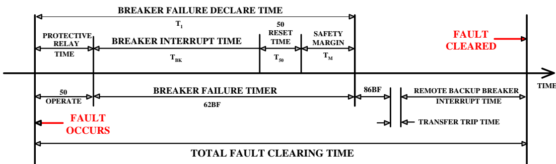
Figure 3.8.3 — Example of Breaker Failure Timing Chart 3
