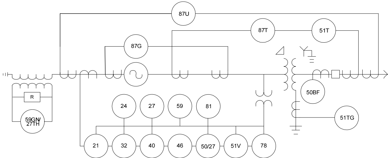
Figure 1.1 — Relay Configuration
