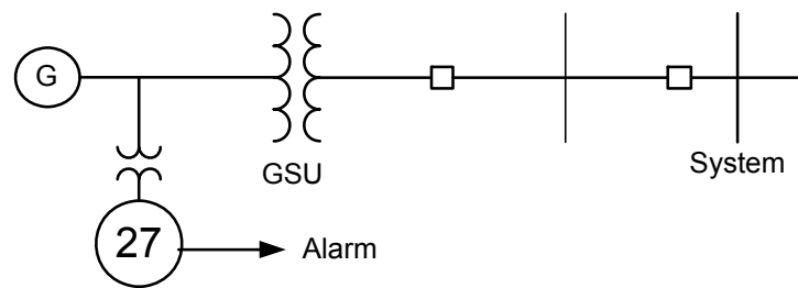
Figure 3.3.1.1 — Typical Unit Generator Undervoltage Scheme
