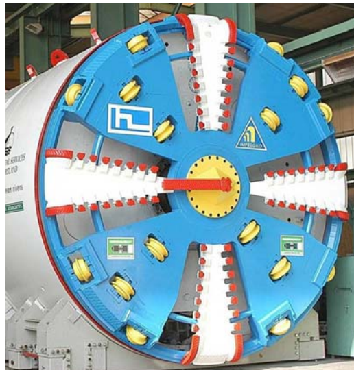
Figure 7-6 Slurry Face Tunnel Boring Machine (SFM) (courtesy of Herrenknecht).
