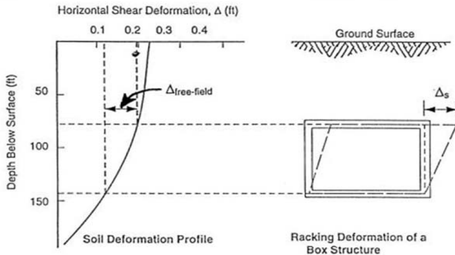
Figure 13-20 Soil Deformation Profile and Racking Deformation of a Box Structure
