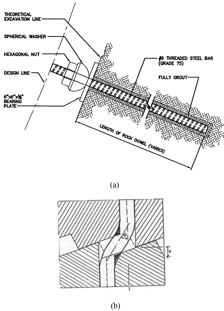
Figure 6-17 (a) Temporary Rock Dowel; (b) Schematic Function of a Rock Dowel under Shear
