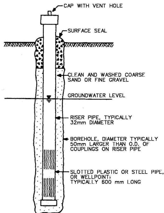
Figure 15-29 Schematic of Observation Well (After Dunnycliff, 1988, 1993)
