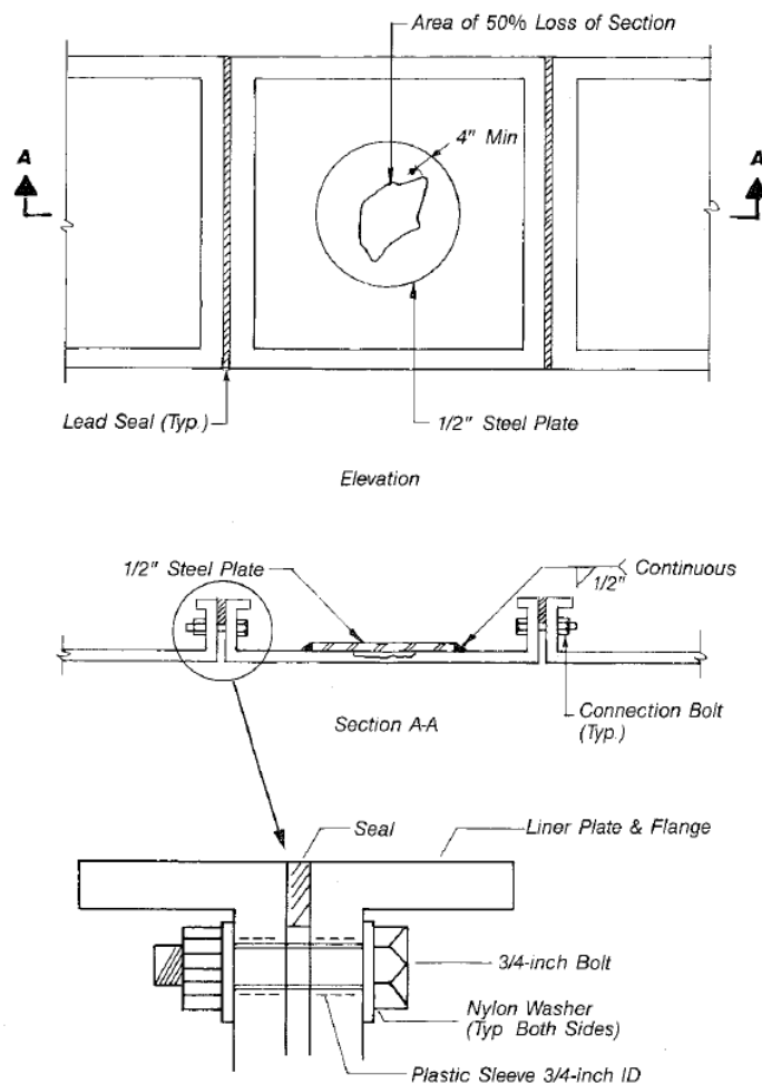
Figure 16-15 Steel Segmental Liner Repair (Russell, 2000)
